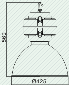
SD2a-G-1 (45W/85W)
