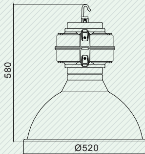
SD2a-G-2 (125W/155W/210W)
