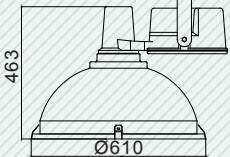
SD7a-G-3 (125W/155W/210W)
