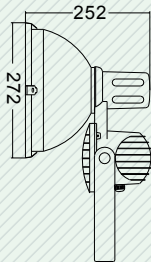
SD7a-G-1 (45W)
